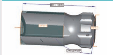
Mining industry drill bit reverse engineered by scanning
